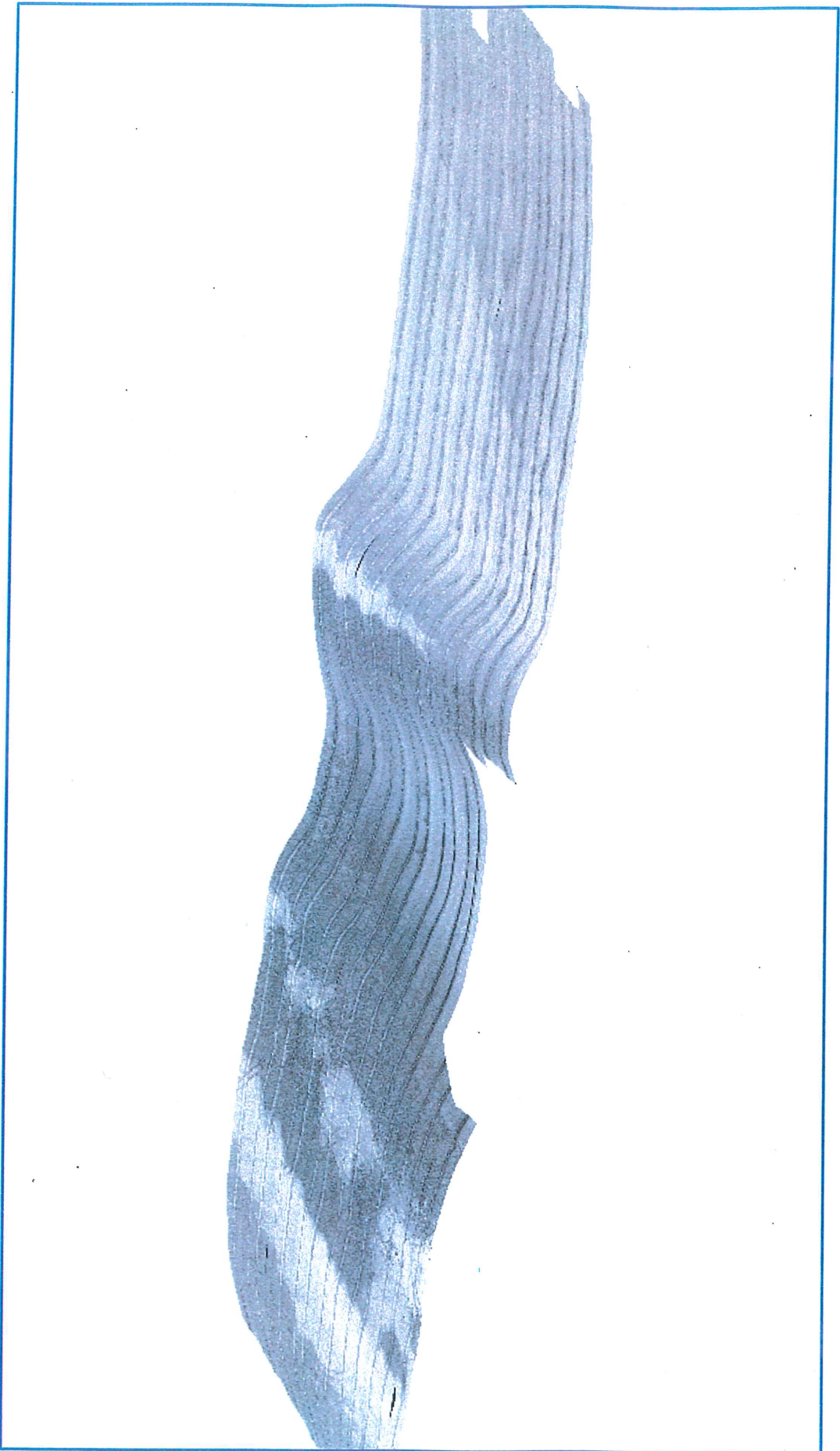
Figure 22. Very-high resolution image of the central part of the southern zone based on the combination of side-scan sonar and multibeam data (March 2000).
