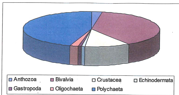
Figure 26. Relative abundances of the dominant taxa in the study area
