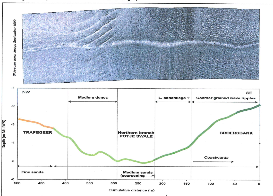
Figure 38. Demonstration of the relation of sediment texture with the observed reflectivity on side-scan sonar imagery. Additionally, the corresponding bathymetric profile is given.
