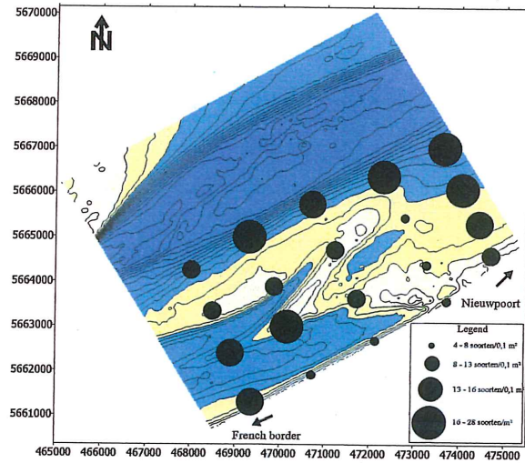
Figure 10. Distribution of the macrobenthic diversity (Degraer et al. , 1999).
