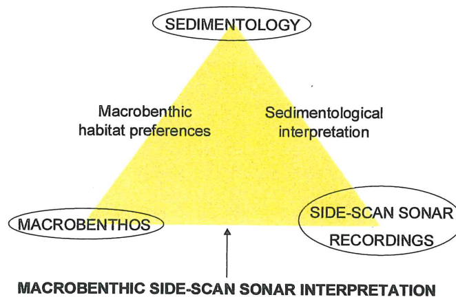
Figure 36. The concept of the macrobenthic side-scan sonar interpretation
