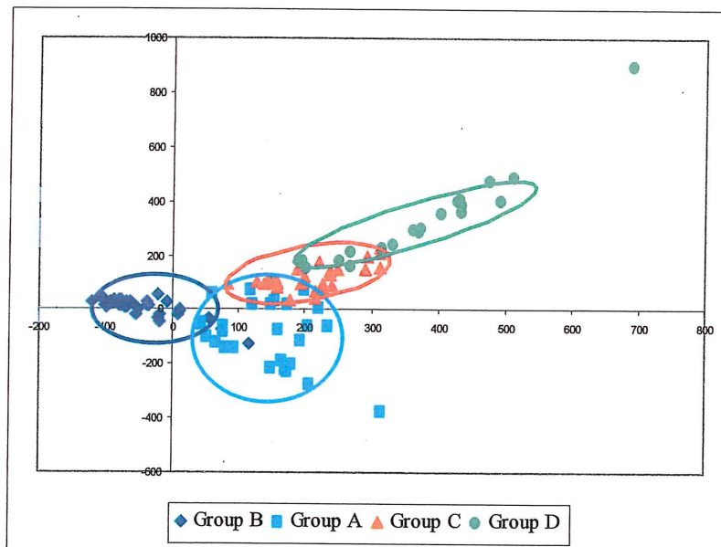
Figure 33. CA of the macrobenthic samples of March 2000, with the presentation of the four station groups (A, B, C and D)
