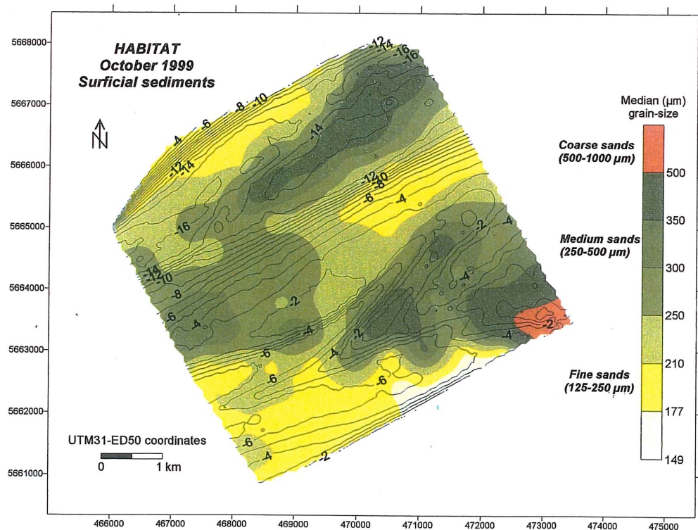
Figure 19. Contour map of the median grain-size of the surficial sediments (October 1999).
