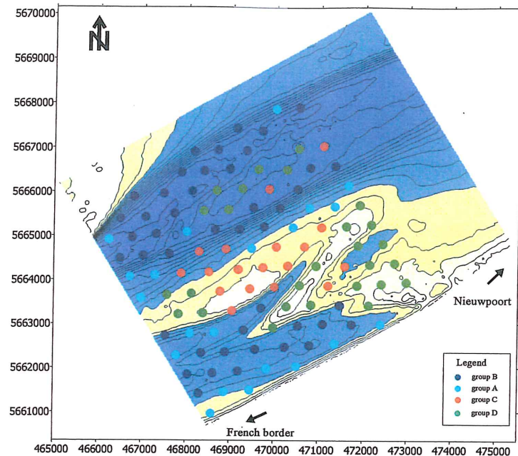
Figure 28. The spatial distribution of the four station groups in the study area
